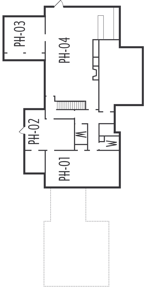
LOWER LEVEL PLANS POTTERS HOUSE
